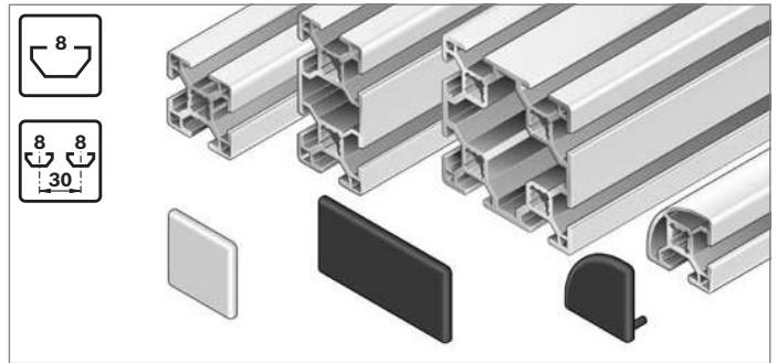
Nut 8 mm, Raster 30
